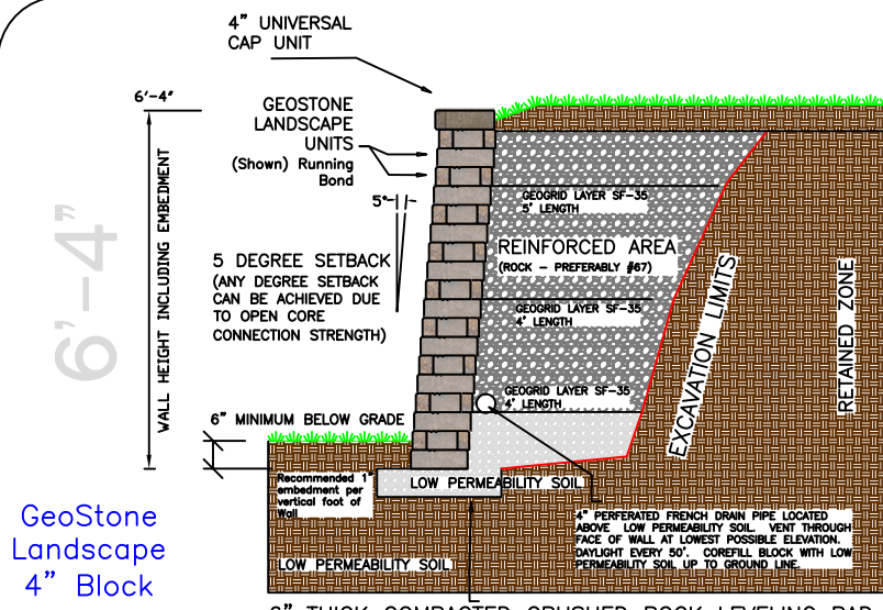
Typical Reinforced GeoStone Retaining Wall
