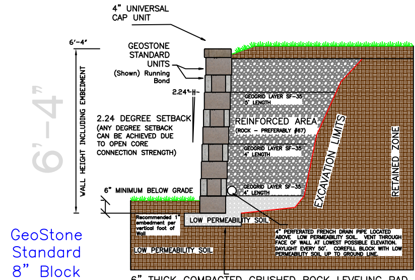
Typical Reinforced GeoStone Retaining Wall
