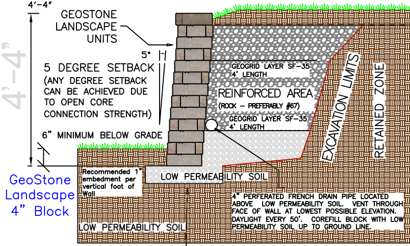
Typical Reinforced GeoStone Retaining Wall
