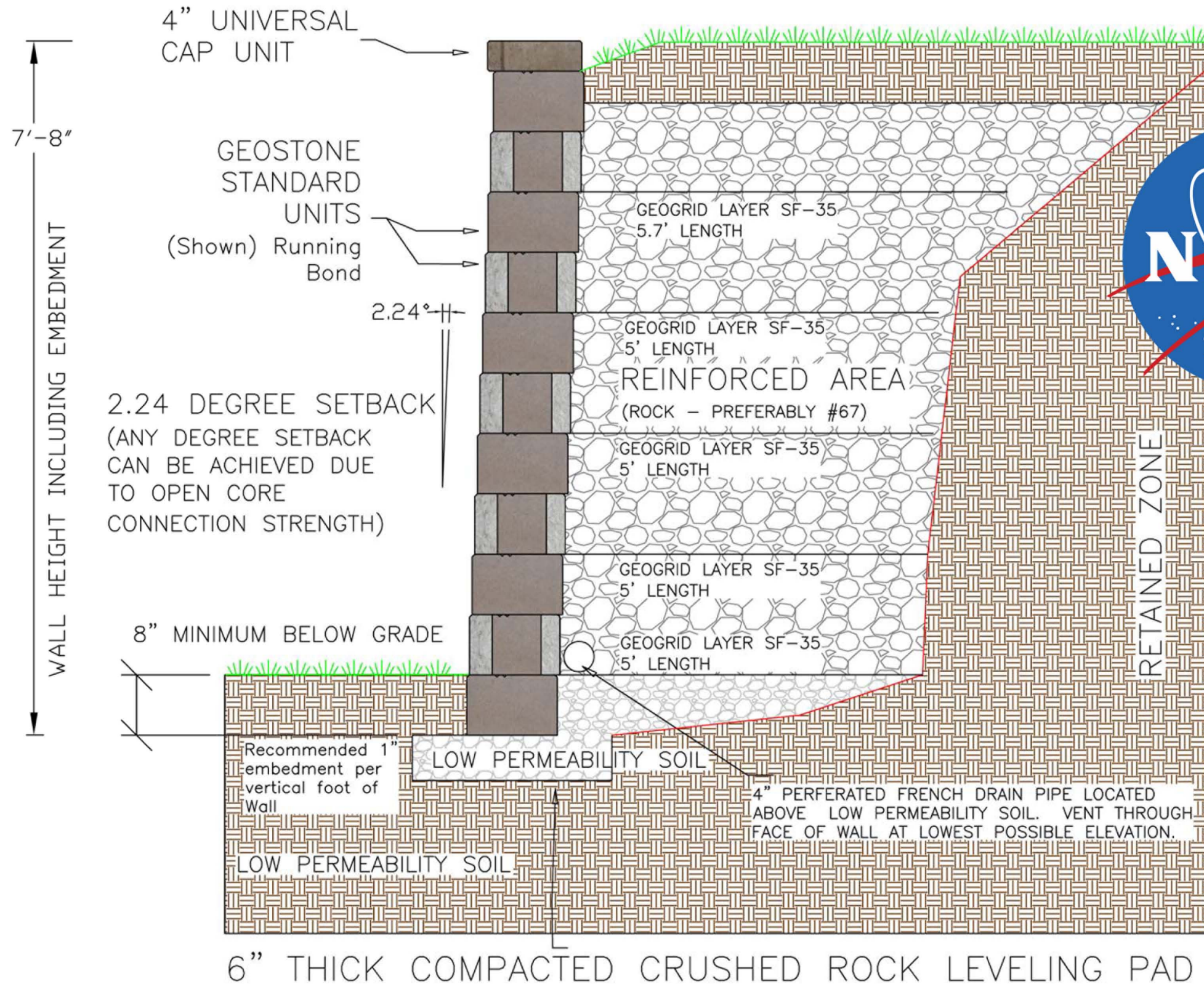
Typical Reinforced GeoStone Retaining Wall
